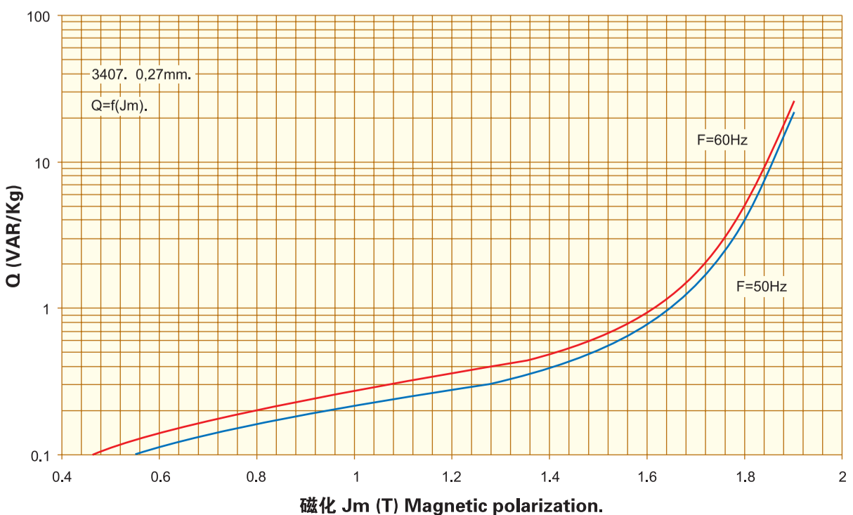
无功功率. Reactive Power. Q=f(J_m) , 0,27mm. 3407
