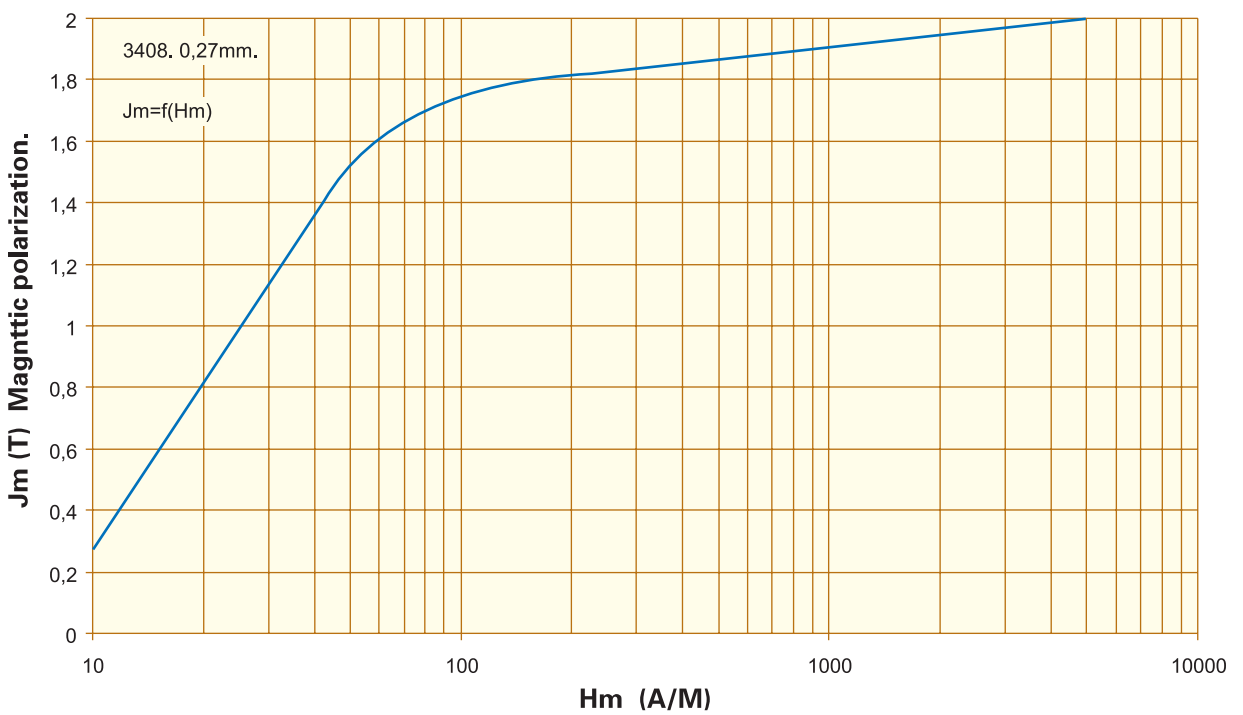
磁化曲线 Magnetic polarization. J_m=f(H_m) , F=50\text{Hz} . 0,27mm. 3408
