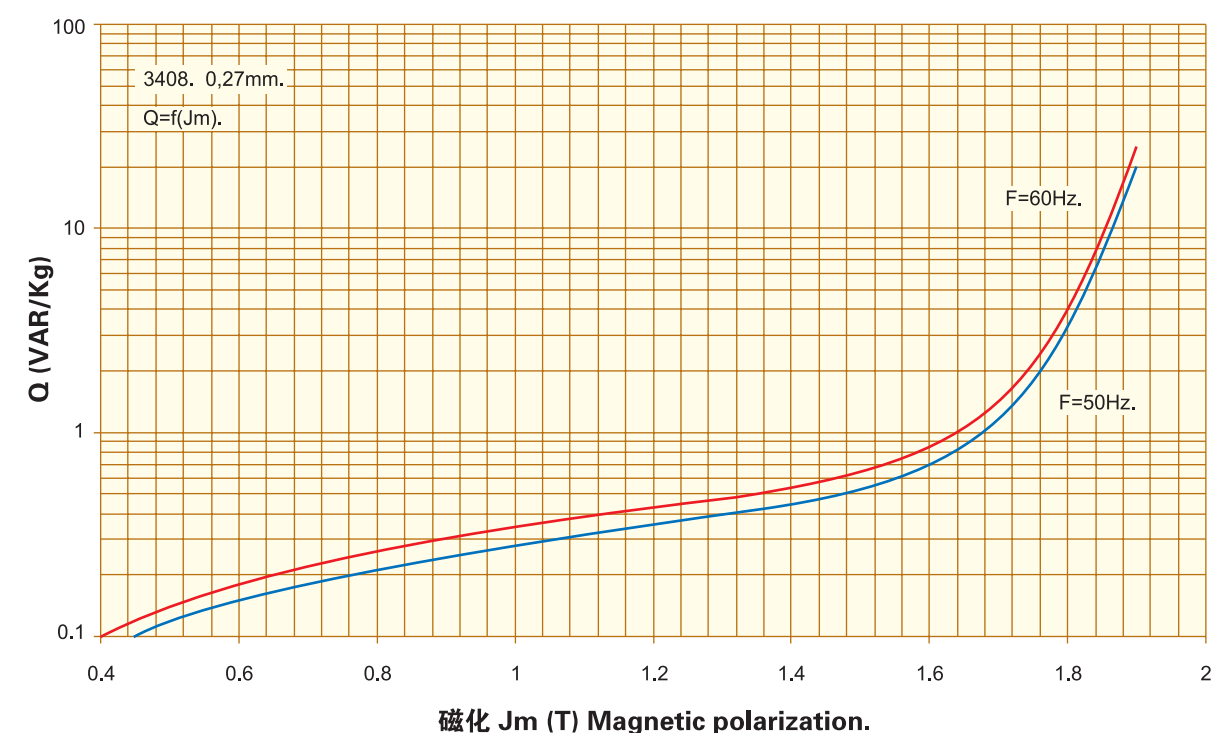
无功功率. Reactive Power, Q=f(J_m) , 0,27mm. 3408
