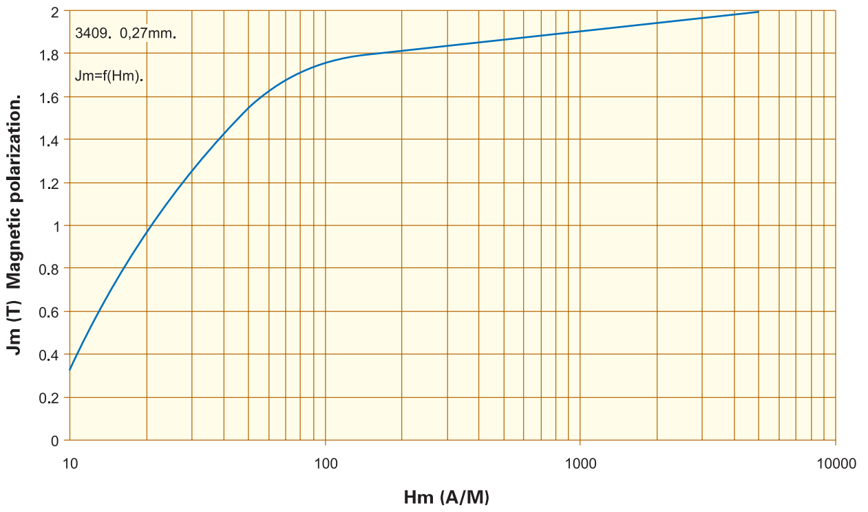
磁化曲线 Magnetic polarization. J_m=f(H_m) , F=50\text{Hz} . 0,27mm. 3409.
