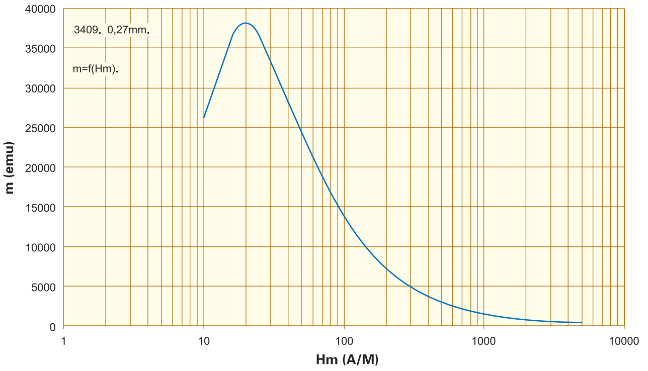
相对导磁率 Relative peak permeability. m=f(H_m) , F=50\text{Hz} . 0,27mm, 3409
