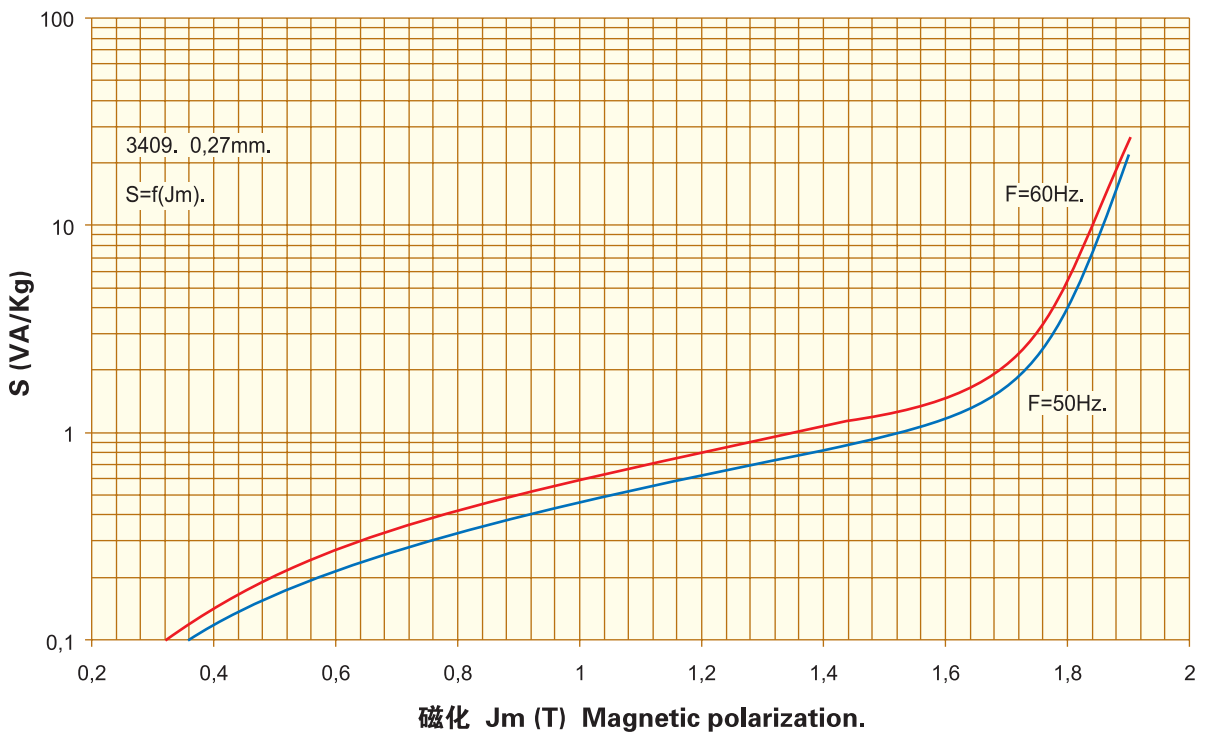
激磁功率 Exciting Power. S=f(J_m) , 0,27mm. 3409.
