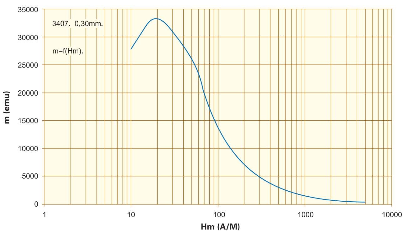
相对导磁率. Relative peak permeability. m=f(H_m) , F=50\text{Hz} . 0,30mm. 3407
