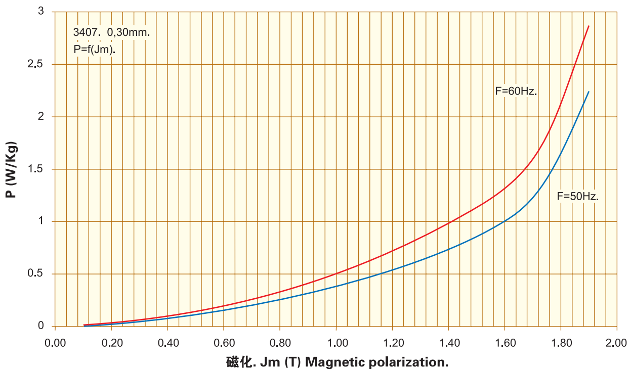
磁损耗. Specific Core Loss, P=f(J_m) , 0,30mm. 3407.
