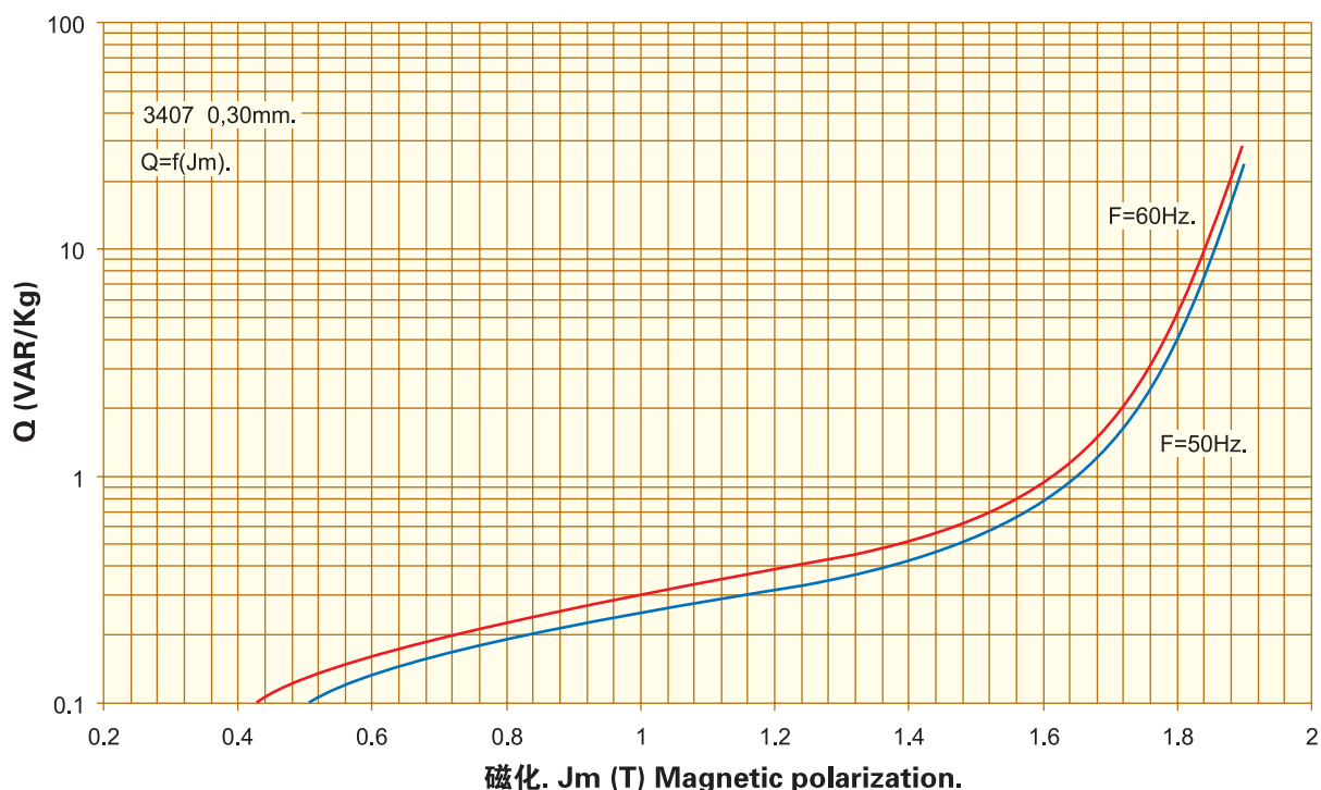
无功功率. Reactive Power. Q=f(J_m) , 0,30mm, 3407
