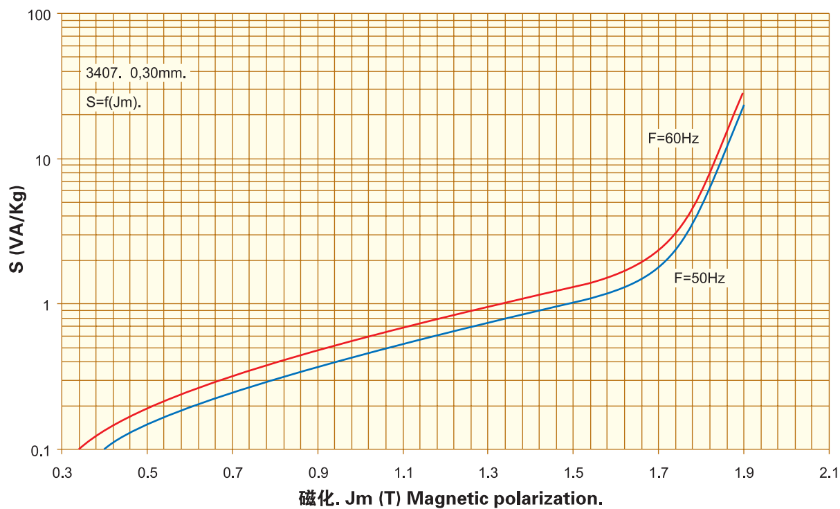
激磁功率. Exciting Power. S=f(J_m) , 0,30mm. 3407
