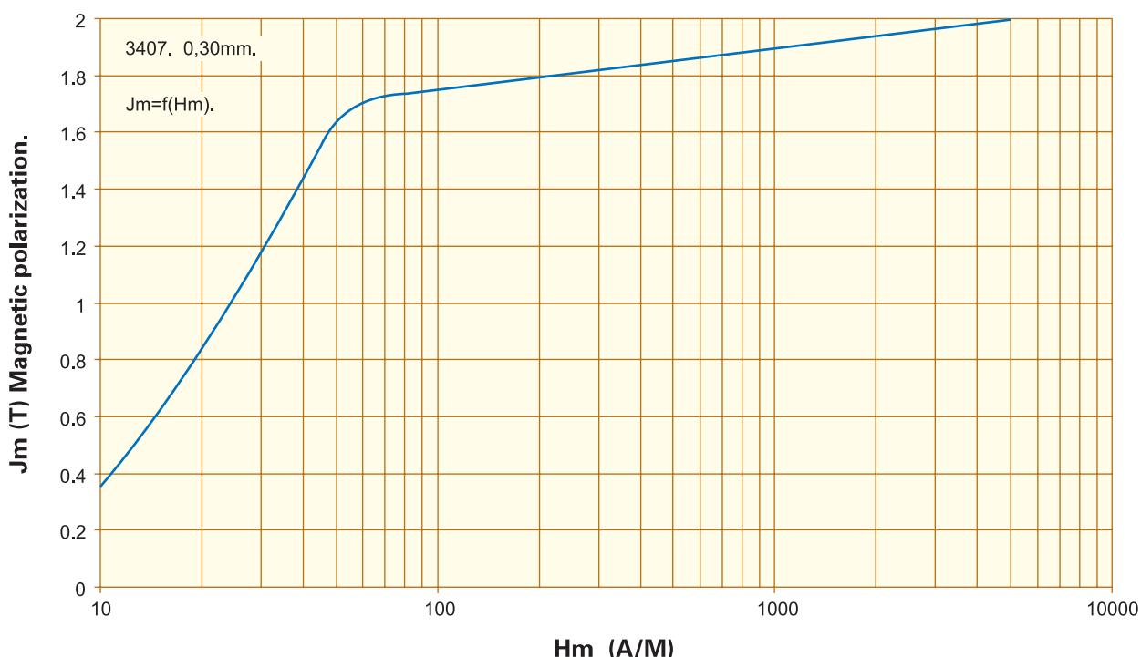
磁化曲线 Magnetic polarization. J_m=f(H_m) , F=50\text{Hz} . 0,30mm. 3407
