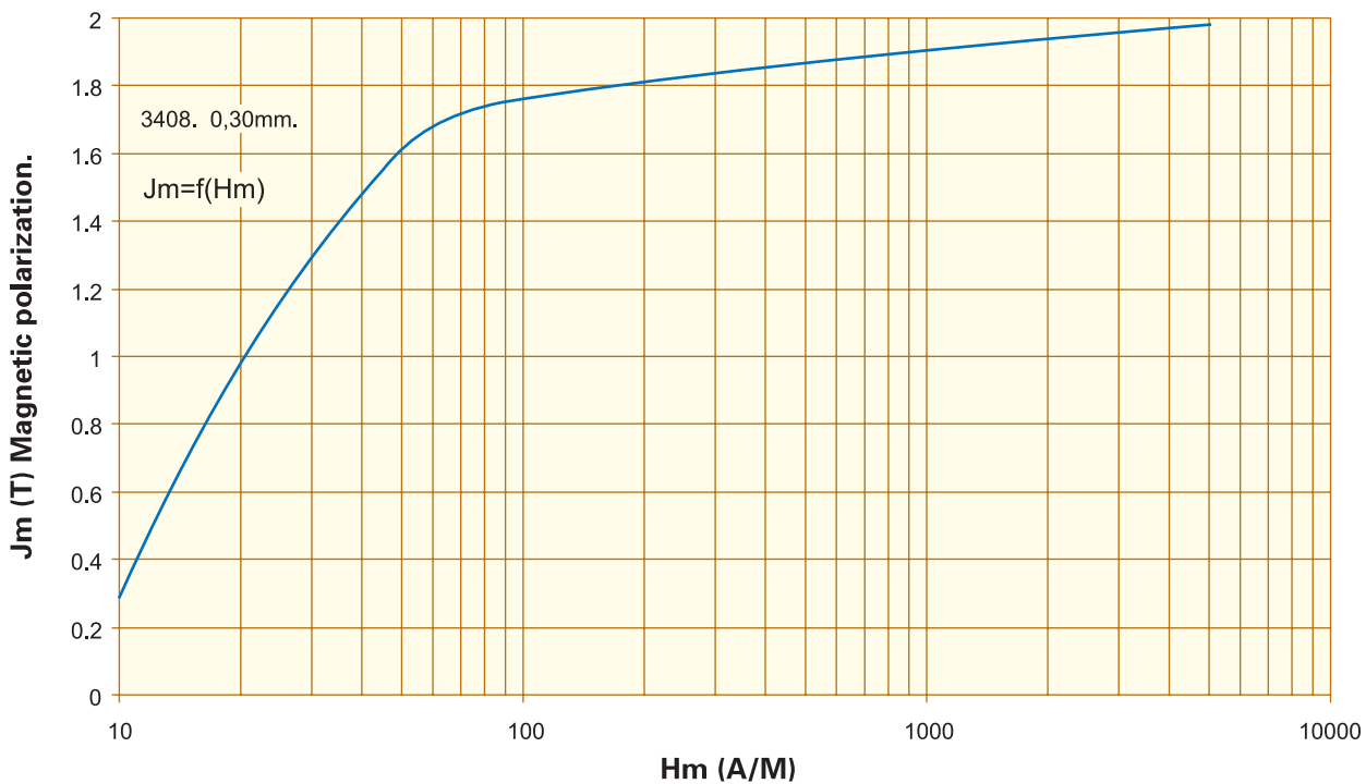
磁化曲线 Magnetic polarization. J_m=f(H_m) , F=50\text{Hz} . 0,30mm. 3408.
