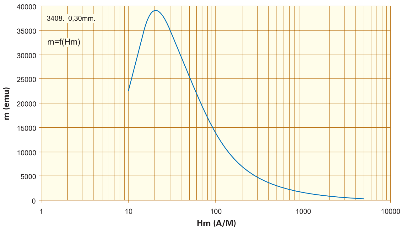
相对导磁率 Relative peak permeability. m=f(H_m) , F=50\text{Hz} . 0 30mm. 3408.
