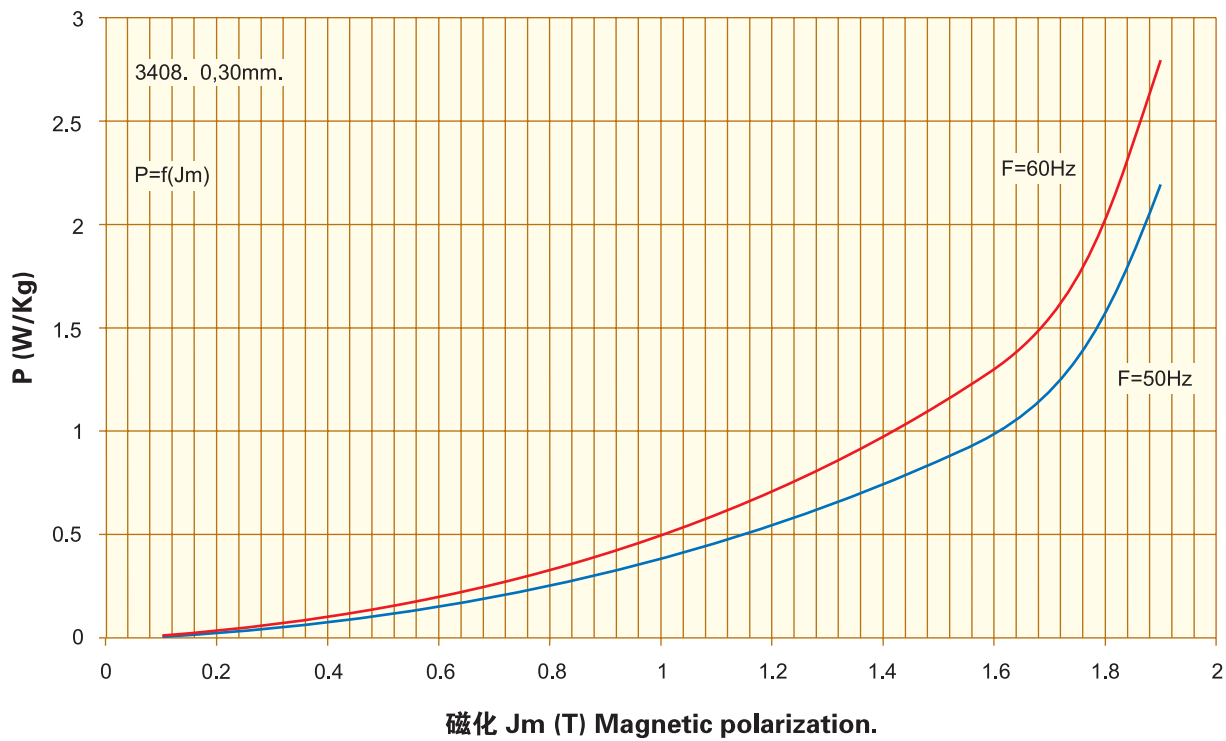
磁损耗. Specific Core Loss. P=f(J_m) , 0,30mm. 3408.
