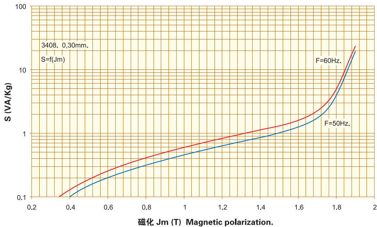
激磁功率. Exciting Power. S=f(J_m) , 0,30mm. 3408.
