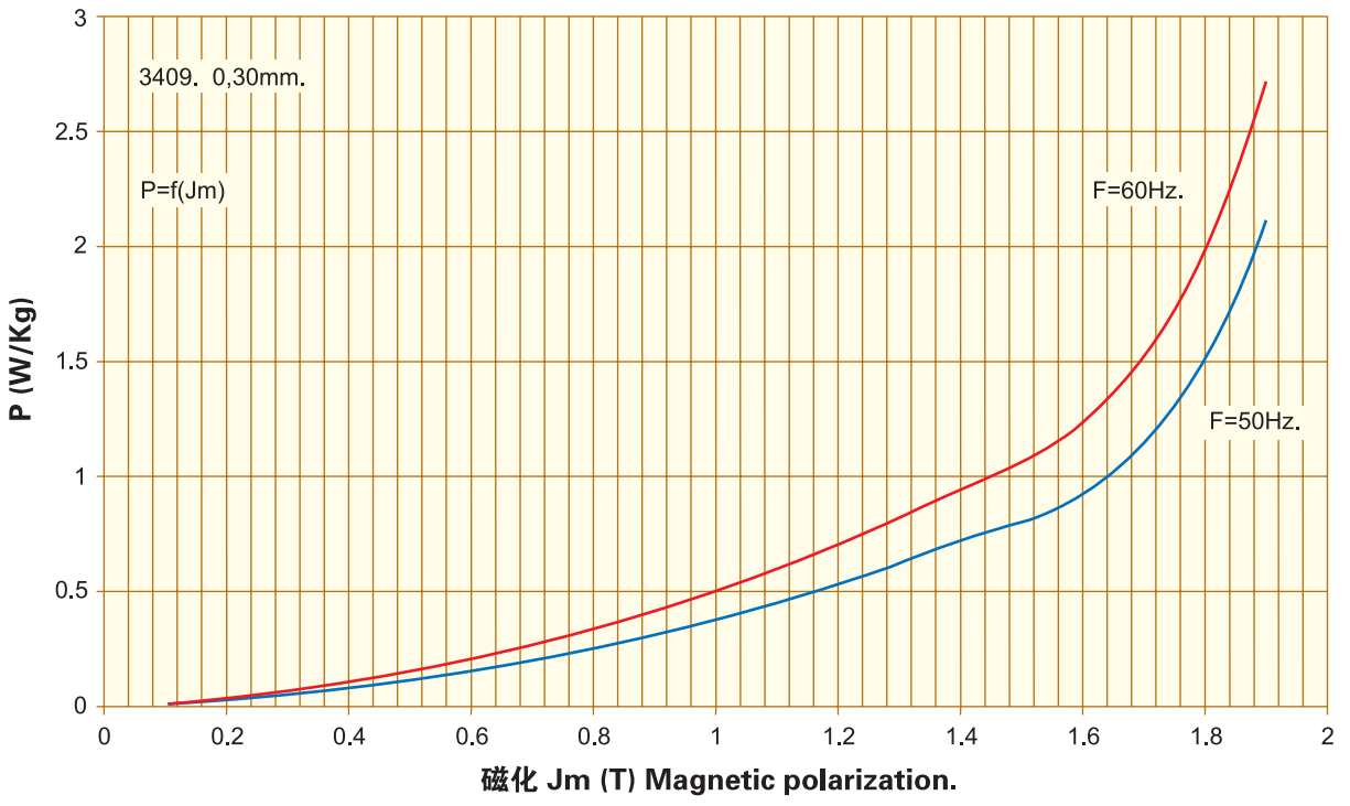
磁损耗 Specific Core Loss. P=f(J_m) . 0,30\text{mm.} 3409
