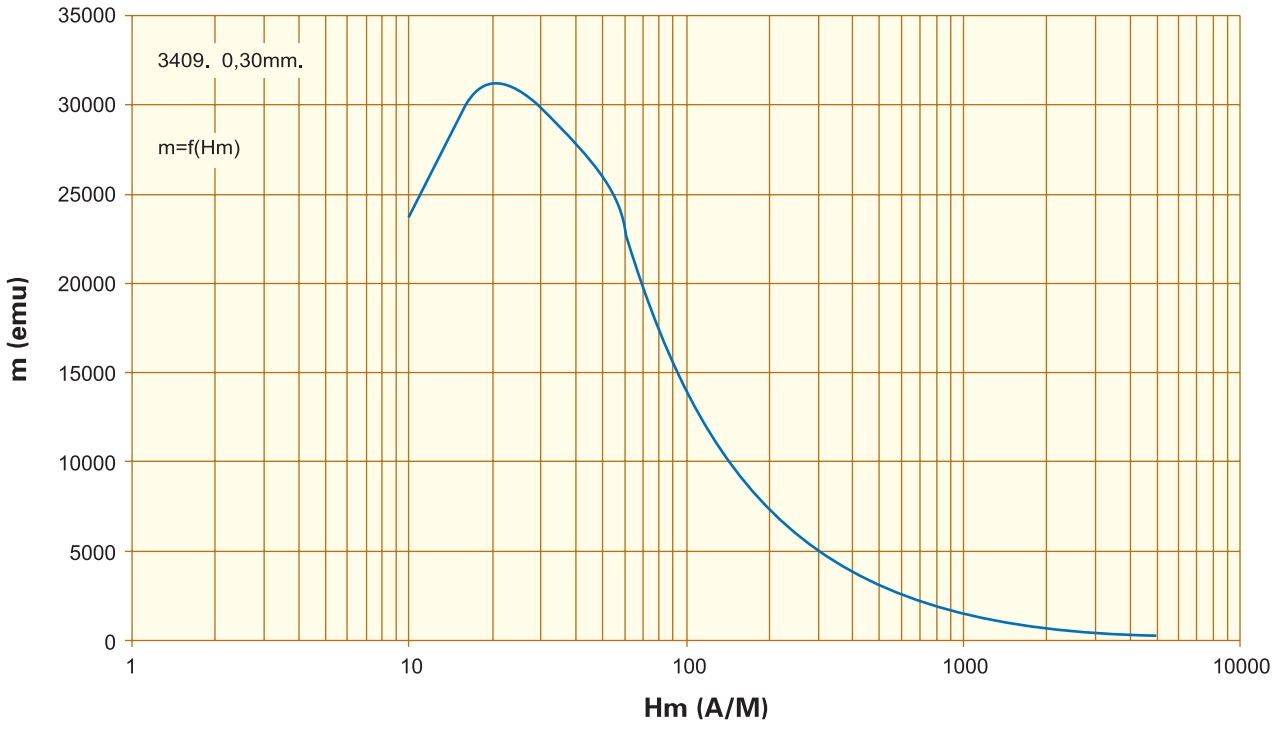
相对导磁率 Relative peak permeability, m=f(H_m) , F=50\text{Hz.} 0,30\text{mm.} 3409.
