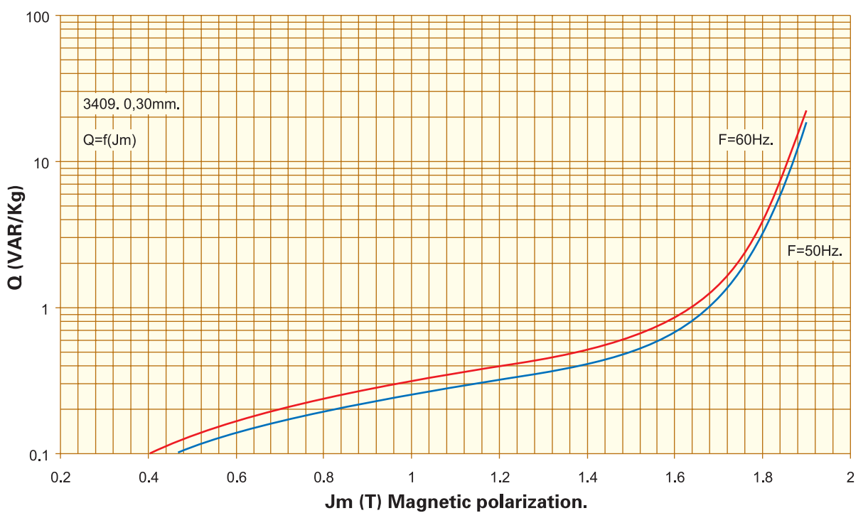
无功功率 Reactive Power. Q=f(J_m) . 0,30\text{ mm} 3409.
