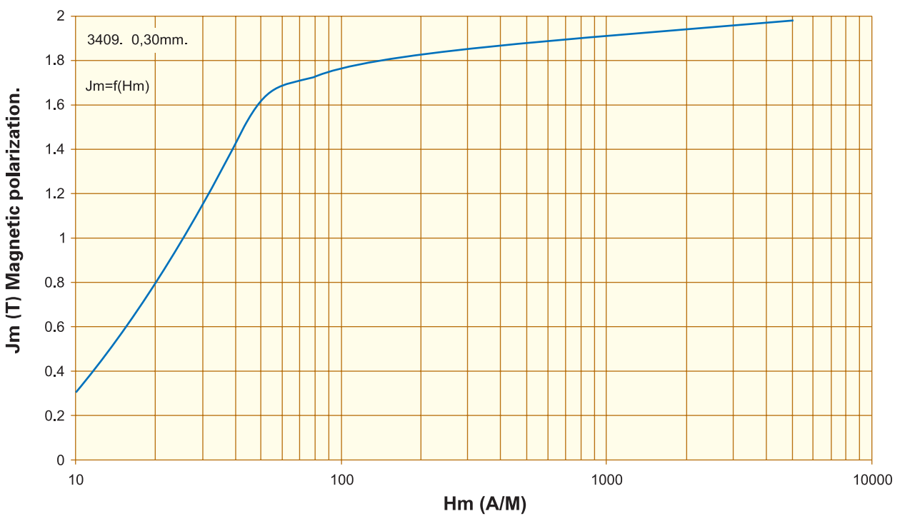
磁化曲线 Magnetic polarization. J_m=f(H_m) , F=50\text{Hz.} , 0,30\text{mm.} 3409
