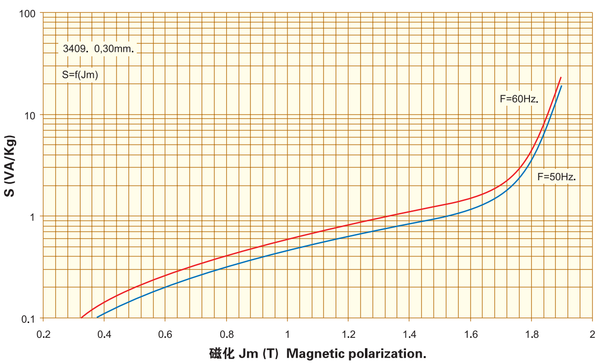
激磁功率 Exciting Power. S=f(J_m) , 0,30\text{mm.} 3409.
