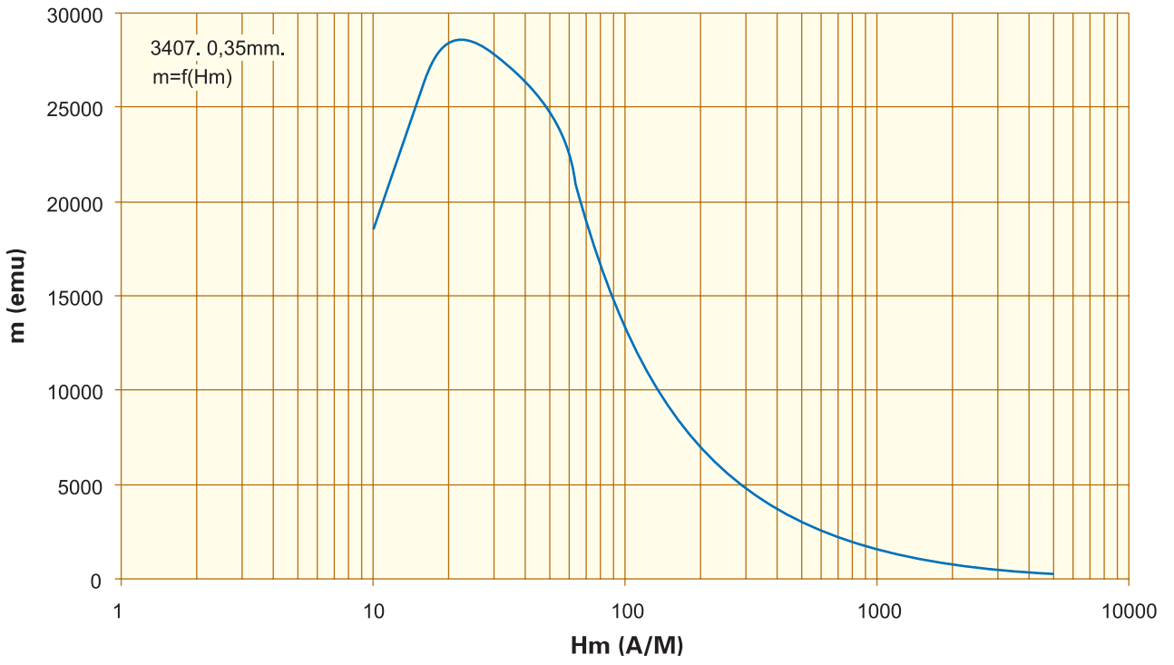
相对导磁率 Relative peak permeability. m=f(H_m) , F=50\text{Hz} . 0,35mm. 3407
