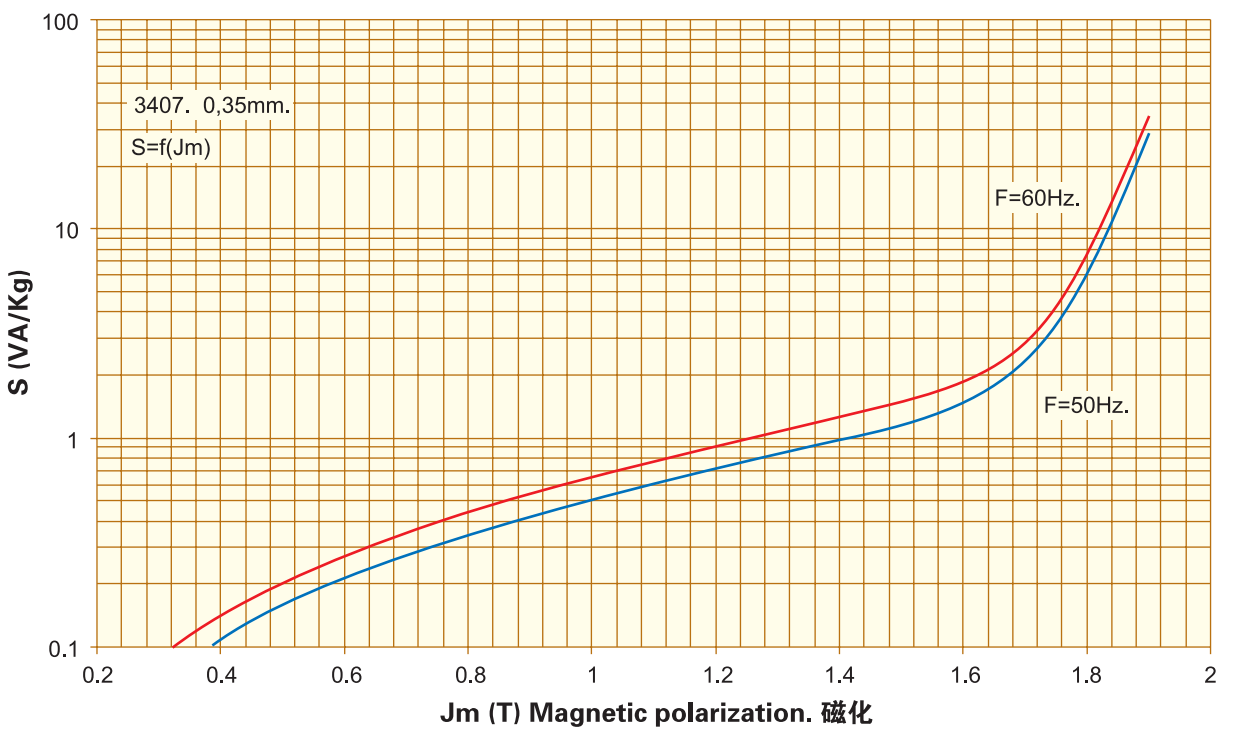
激磁功率. Exciting Power. S=f(J_m) , 0,35mm. 3407
