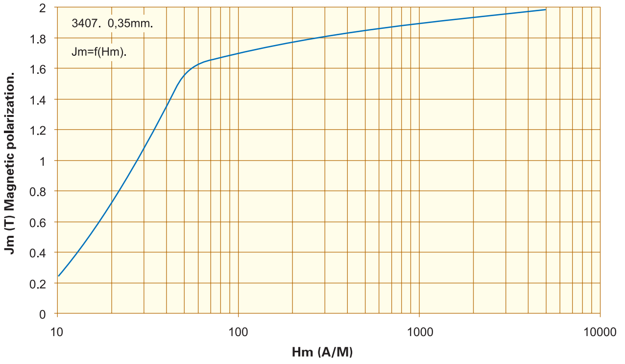
磁化曲线 Magnetic polarization. J_m=f(H_m) , F=50\text{Hz} . 0,35mm. 3407
