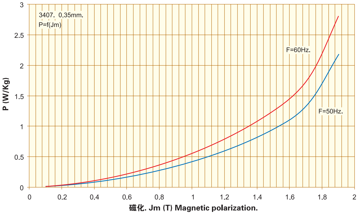
磁损耗. Specific Core Loss. P=f(J_m) , 0,35mm. 3407
