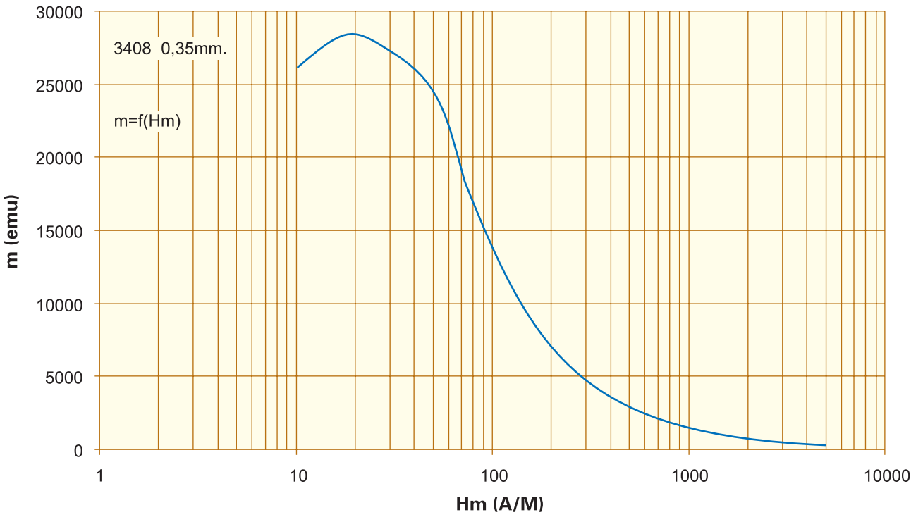
相对导磁率 Relative peak permeability. m=f(H_m) , F=50\text{Hz} . 0,35mm. 3408.
