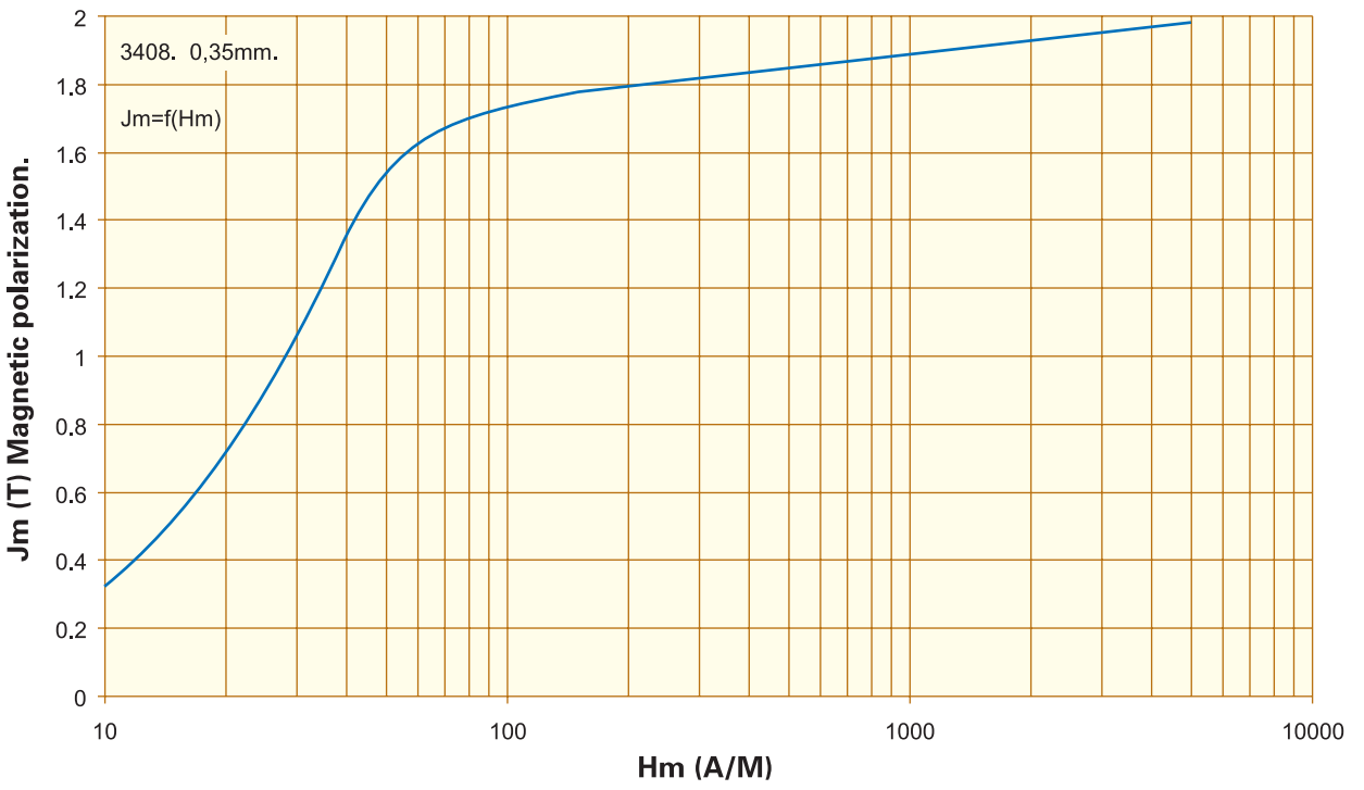
磁化曲线 Magnetic polarization. J_m=f(H_m) , F=50\text{Hz} . 0,35mm, 3408.
