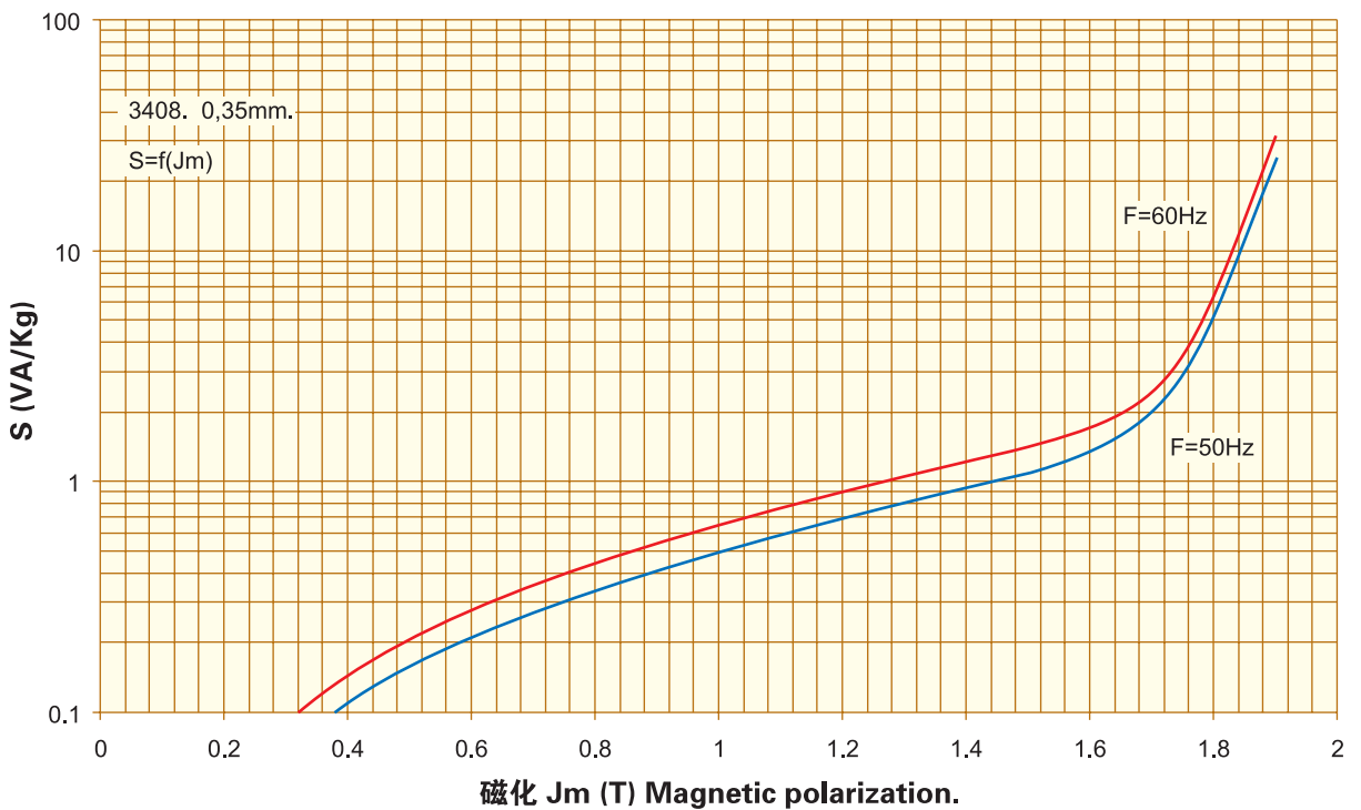
激磁功率. Exciting Power. S=f(J_m) , 0,35mm. 3408.
