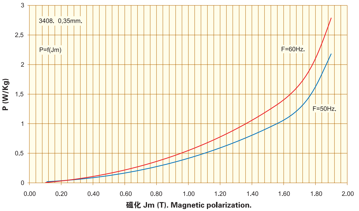
磁损耗. Specific Core Loss. P=f(J_m) , 0,35mm. 3408.
