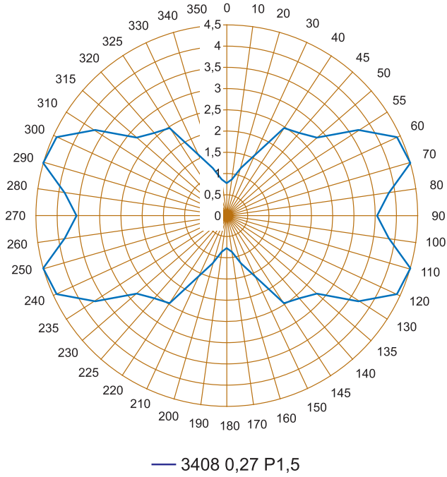
角位置单位铁损 Specific core loss at an angle to rolling direction, P1,50/70
