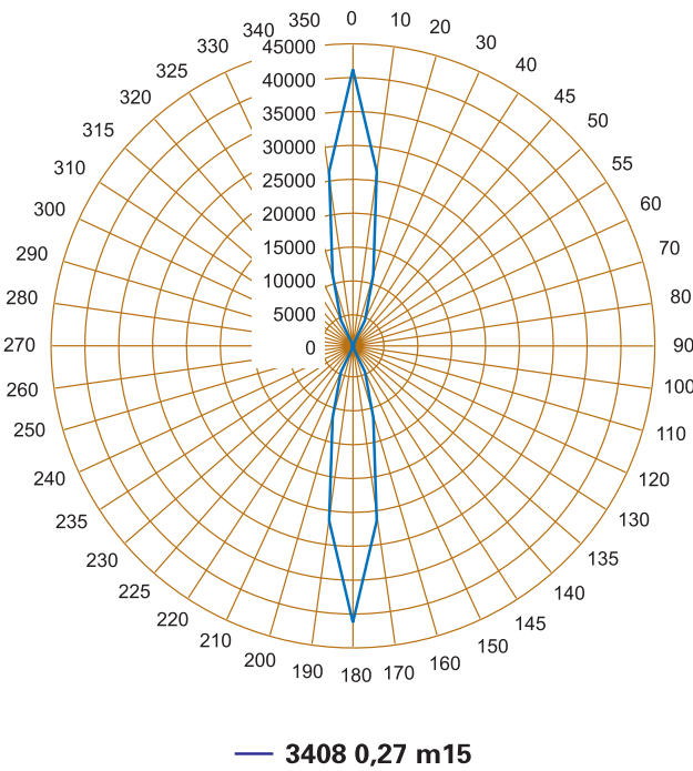
角位置磁导率 Permeability at an angle to rolling direction, \mu 1,5
