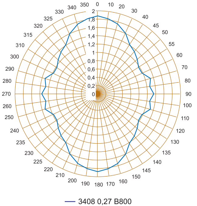
角位置磁感 Magnetic induction at an angle to rolling direction, B800
